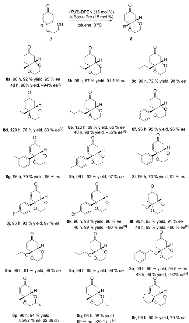
Scheme 3. Organocatalytic enantioselective intramolecular oxa-Michael reaction. Reaction conditions: ( R,R )-DPEN (15 mol %) and N -Boc-L-Pro (15 mol %) in toluene (0.5 M) at 0 °C for 96–120 h. [a] Catalyst 6 (20 mol %) and N -Boc-L-Phe (20 mol %) in CH 2 Cl 2 (0.5 M) at room temperature for 48 h. [b] o -fluorobenzoic acid was used. [c] 7p was prepared from ( R )-1,2-propylene glycol. Yields shown are of isolated products. Enantiomeric excesses were determined by HPLC analysis on a chiral stationary phase. The diastereomeric ratios were determined by 1 H NMR spectroscopy of the crude reaction mixture.
